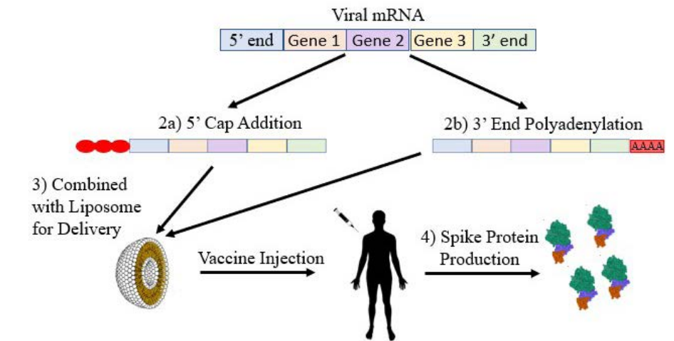
Figure 1: Structural modification and translation of mRNA vaccines. The transcription of mRNA for the vaccines occurs in vitro using a cDNA template and gets stabilized through either adding a 5' cap (2a) or polyadenylation (2b). This processed and stabilized RNA is transferred into the host cell via a liposome (3) where the functional mRNA is translated into antigenic spike proteins (4).
