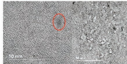
Figure 6: TEM shows small colloids. The faint appearance of the quantum dot (left) evidences a composition of a light atom such as carbon.
