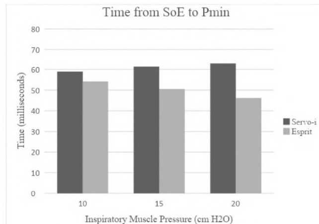
Figure 2. Mean Time from SoE to Pmin. This figure displays the average time from the start of an inspiratory effort to the lowest airway pressure required to trigger ventilator breath delivery. The Respirationes Esprit mechanical ventilator outperforms the Maquet Servo-i under each measure of inspiratory muscle pressure, suggesting that it is superior in spontaneous breath detection.
